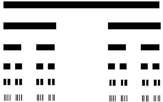
Figure 1: Cantor dust - each of the lines has the same fractal dimension (0.6309) but a different texture, which is dependent on how many times the replacement rule (remove the central third of each line segment) has been applied. For illustrative purposes, the lines have been thickened.
